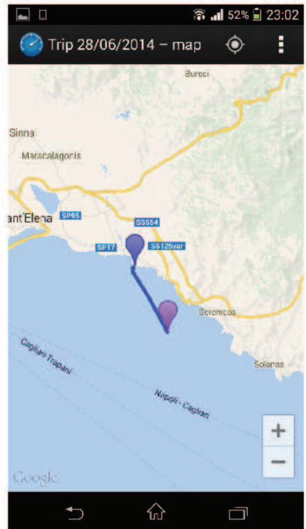
Distance: Dive Position- -Emergency Location
